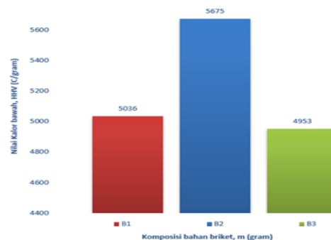
Gambar 2. Nilai kalor
